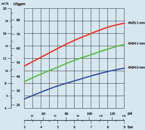
Pressure/Flow
