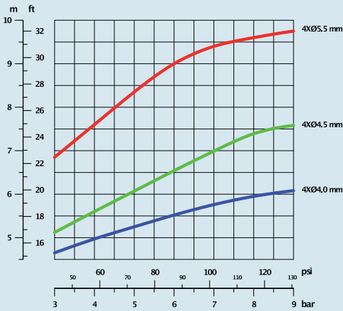
Jet length
